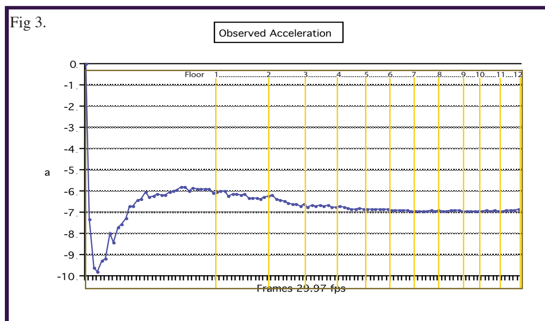
Fig 3. is a plot of observed Acceleration of the roof line. Often said to be 'near free-fall,' in-fact has this profile. There is a reasonably rapid Acceleration decrease over the first 0.6 of a second, (the Floor 1 line is at frame 34 1.033 seconds into the collapse) from here to Floor 1, Acceleration is constant around -6 m/s/s, Acceleration then begins to slowly increase before becoming constant at -6.9 m/s/s, or 70% free-fall shortly after Floor 4. The top block is always accelerating and never decelerating.
