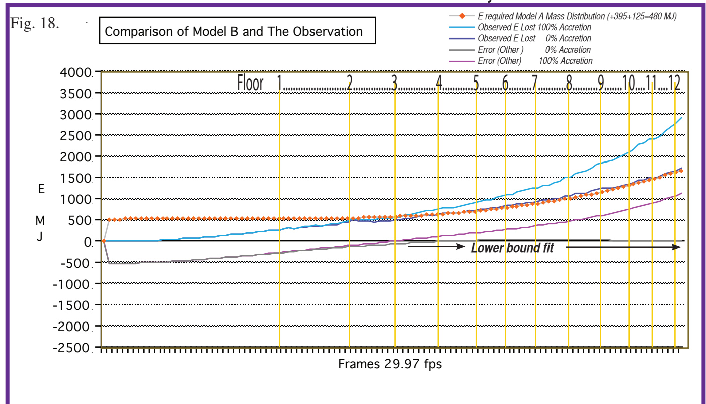
Fig 18 fit with lower bound - 0% Accretion
